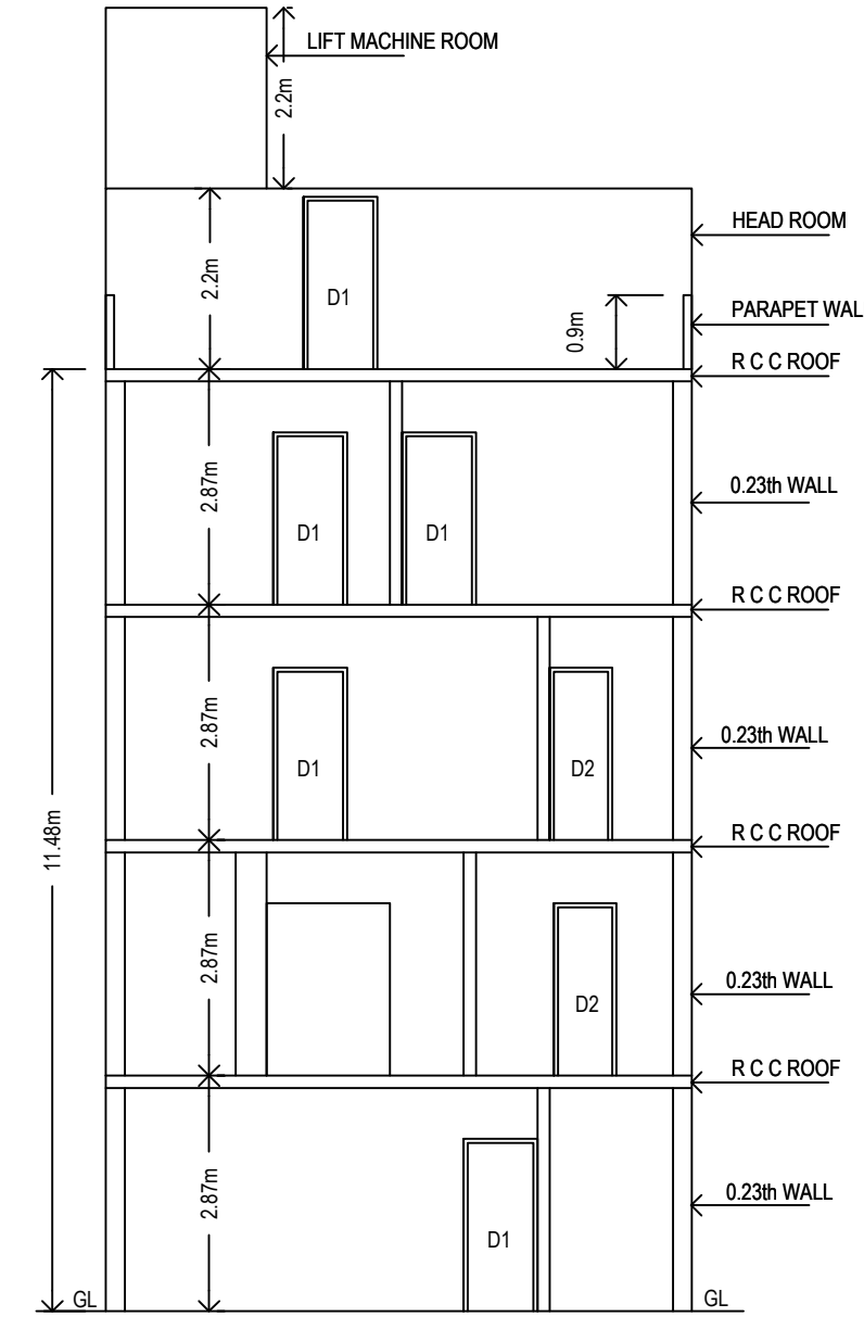
SECTION @ X-X
